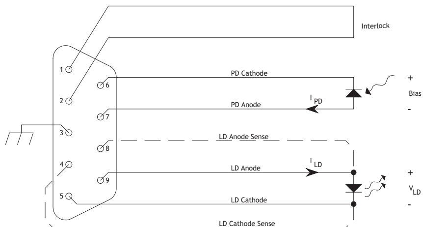
Figure 2.2: Wiring diagram for the Laser Diode. Pin 3 is internally connected to the chassis, and can be used for cable shielding. When the “dashed” connections are made, V_{LD} is a 4-wire measurement; otherwise, it is a 2-wire measurement.
